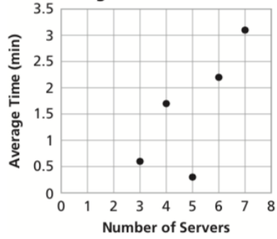
8. a. Relationship between Number of Servers and Average Time to Fill an Order
