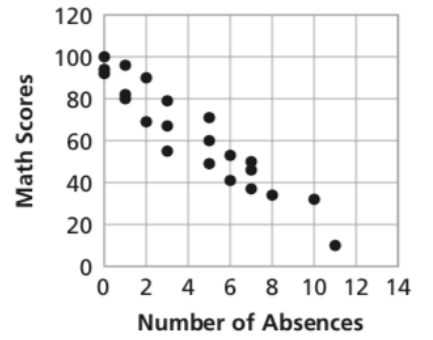
9. a. Number of Absences and Math Scores
