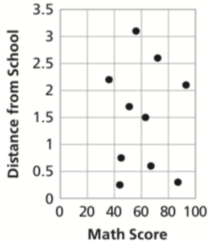
7. a. Relationship between Math Score and Distance from School
